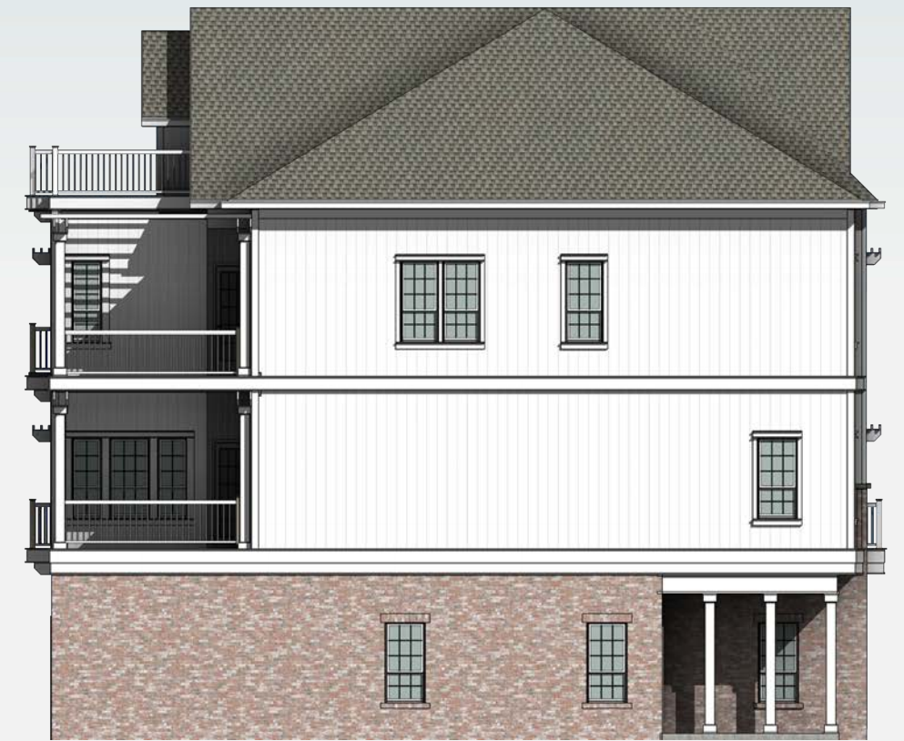
South Elevation
